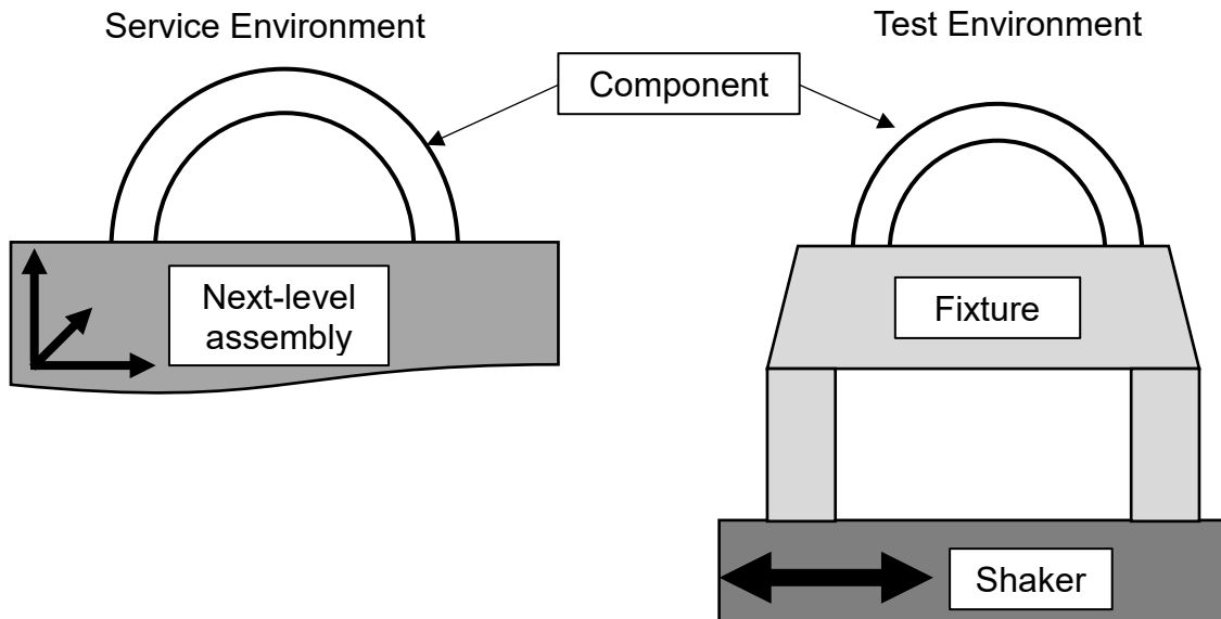
Figure 3.6 Schematic showing a component in the service environment attached to the next-level assembly, and the component in the test environment attached to a fixture on a shaker.
