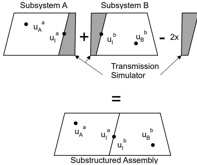
Figure 3.7 Schematic of how a transmission simulator is used in frequency based substructuring.
