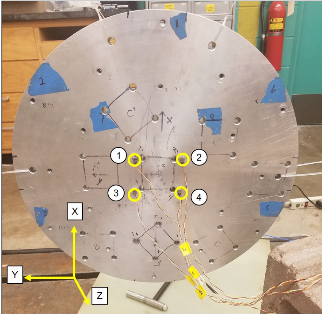
Figure 6.9 Accelerometer placement near interface bolt holes in the center configuration circular plate + impact pad test setup.
