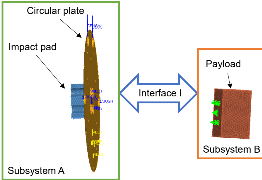
Figure 4.7 Schematic of subsystems and components of the resonant plate finite element model in the application of frequency based substructuring
