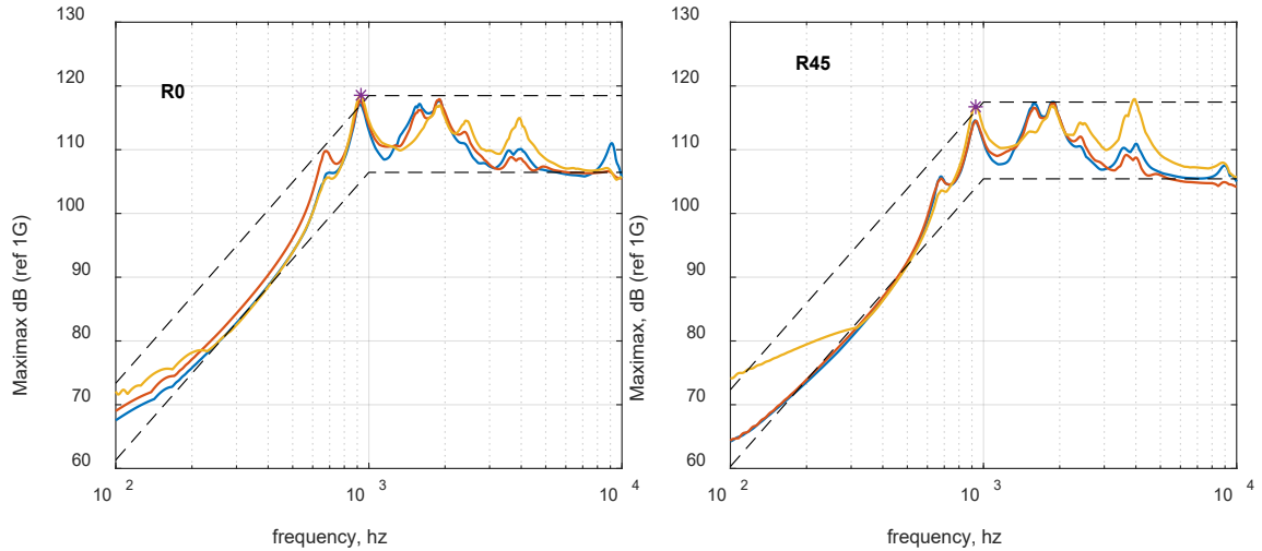
Figure 7.3 Comparison between 0-degree and 45-degree oriented payload SRS for the optimal payload location (-3,3) and response node (9243).
